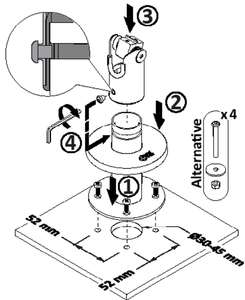
SpacePole® with DuraTilt™ counter mounting
