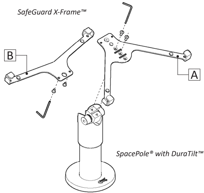
SpacePole® with DuraTilt™ counter mounting
